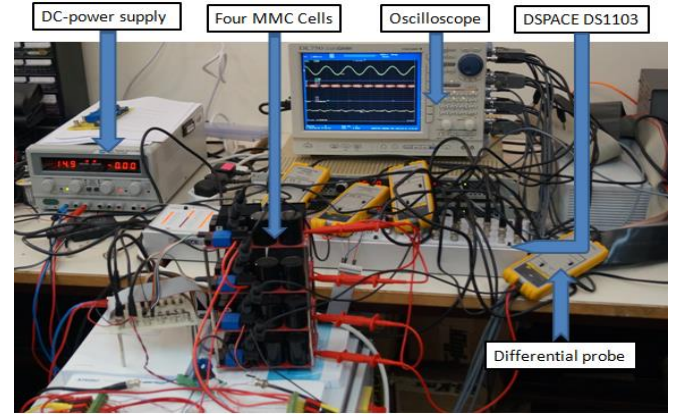
(a) various components of the prototype of 4 cells MMC
