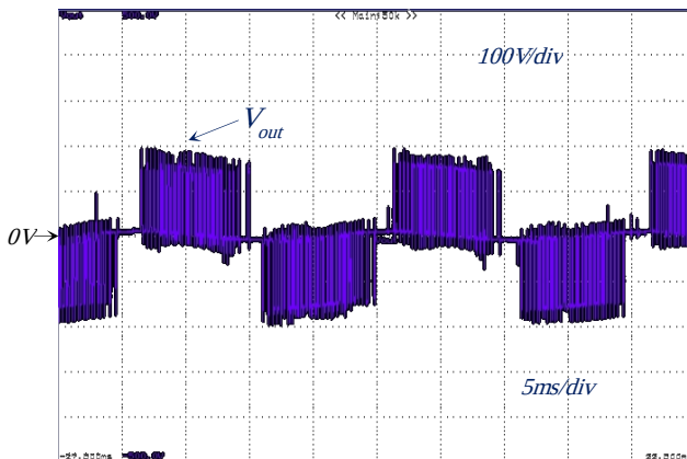
Fig. 15. Experimental results of the three-level output voltage waveforms
