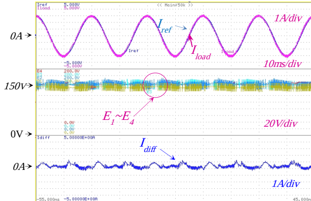
Fig. 14. Experimental results of the proposed WMPC performance with \mu_1 = 2 \times 10^{-2} , \mu_2 = 2 \times 10^{-3} : upper load reference current and actual load current; middle capacitor voltages E1~E4; bottom circulating current
