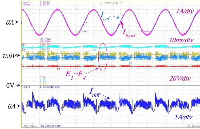
Fig. 13. Experimental results for untuned WMPC: Effect of weighting factors ( \mu_1 = \mu_2 = 10^{-3} ) on the performance of the WMPC. Upper reference and actual load current; middle capacitor voltages E1~E4; bottom circulating current.
