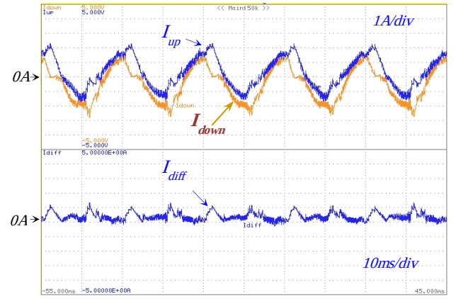
Fig. 16. Experimental results: Upper and lower arm currents (top) and circulating current (bottom)
