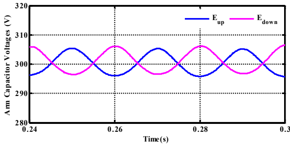
Fig. 7. The sum of upper-arm & lower-arm capacitor voltages waveforms
