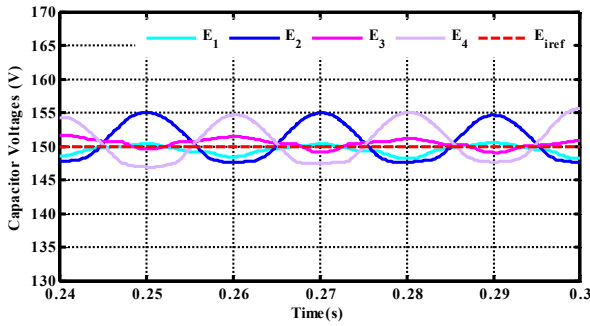
Fig. 6. Capacitor voltages waveforms
