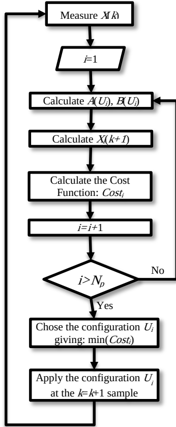
Fig. 4. Flowchart of the proposed WMPC algorithm
