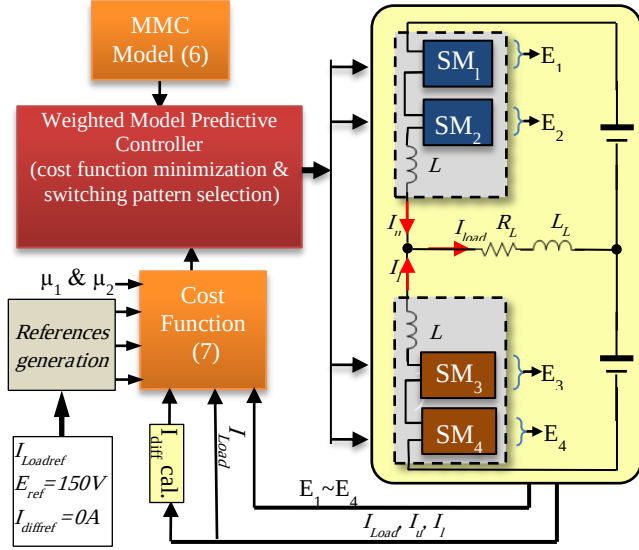
Fig. 3. Proposed controller for the 4-cell MMC
