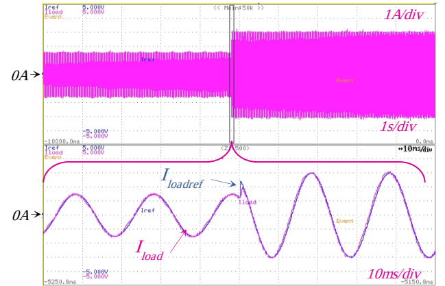
Fig. 17. Experimental results: Transient performance of the WMPC, load reference and actual current are depicted. Lower part is a zoom of the transient instant of the upper waveforms.
