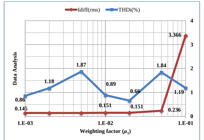
Fig. 5. Variation effect of the weighting factor \mu_1 on the load current THD and rms value of the circulating current.
