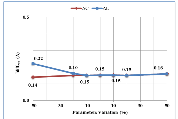
Fig. 11. Sensitivity of the proposed WMPC to the inductor arm variation
