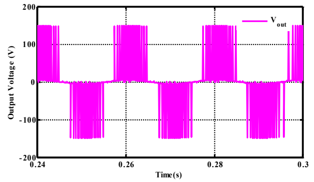
Fig. 10. Output voltage waveform
