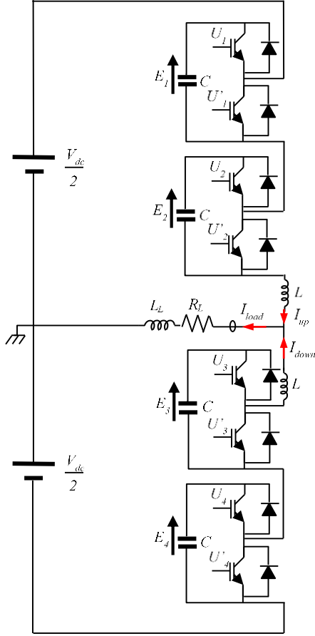
Fig. 2. Configuration of the MMC circuit
