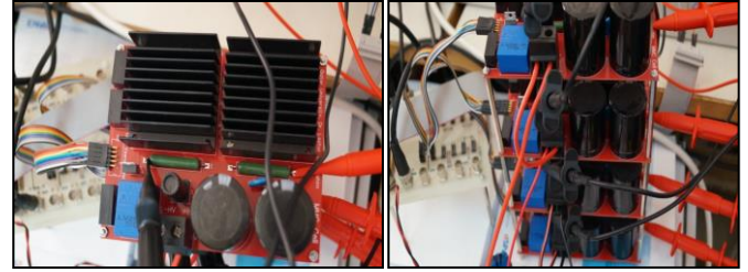
(b) Submodules or Cells of the 3- level MMC inverter
