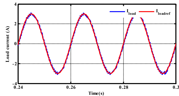
Fig. 8. Load current waveforms
