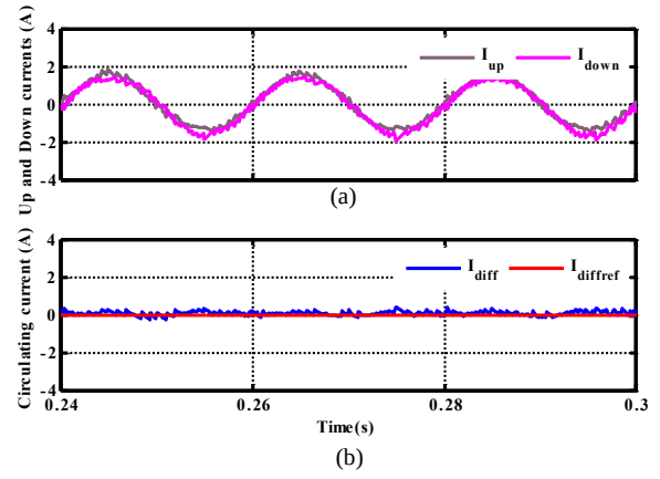
Fig. 9. Current waveforms (a) Upper and lower arm currents; (b) Circulating current
